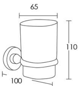
Tumbler Holder ISI58
