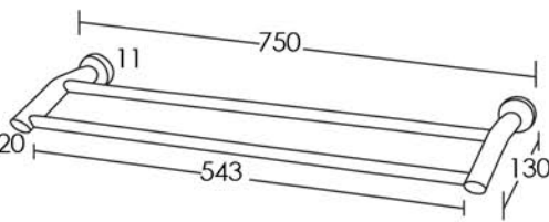
Double Towel Rail ISI61 750mm
