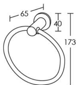
Guest Towel Ring ISI60
