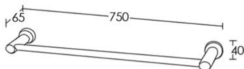
Single Towel Rail ISI30 750mm
