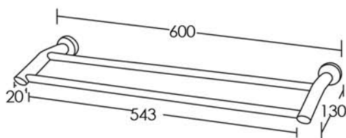
Double Towel Rail ISI48 600mm
