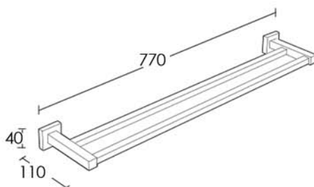
Double Towel Rail QDA61 750mm
