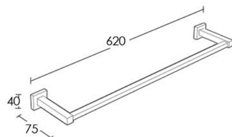
Single Towel Rail QDA24 600mm
