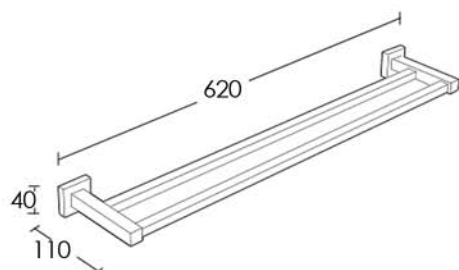
Double Towel Rail QDA48 600mm
