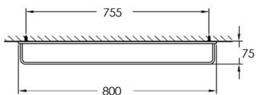
Single Towel Rail ZEN24-2 800mm
