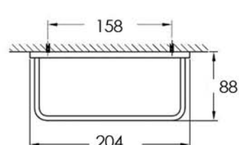
Guest Towel Rail ZEN60
