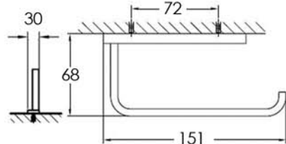
Toilet Roll Holder ZEN51
