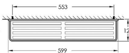
Glass Shelf ZEN53 600mm
