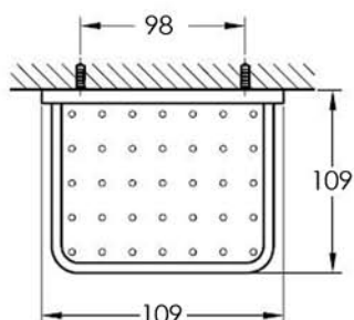
Soap Dish ZEN56 short
