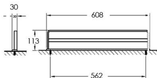
Double Towel Rail ZEN48 600mm
