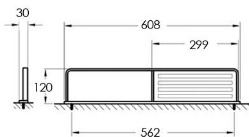
Half Shelf & Rail ZEN53-3
