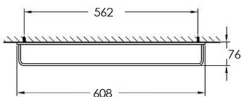
Single Towel Rail ZEN24 600mm
