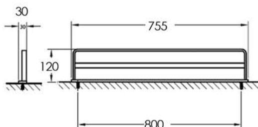
Double Towel Rail ZEN48-2 800mm
