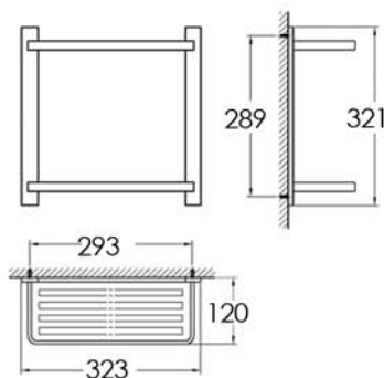
Double Glass Shelf ZEN02
