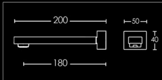
200mm Wall Spout
