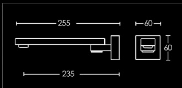
255mm Swivel Wall Spout
