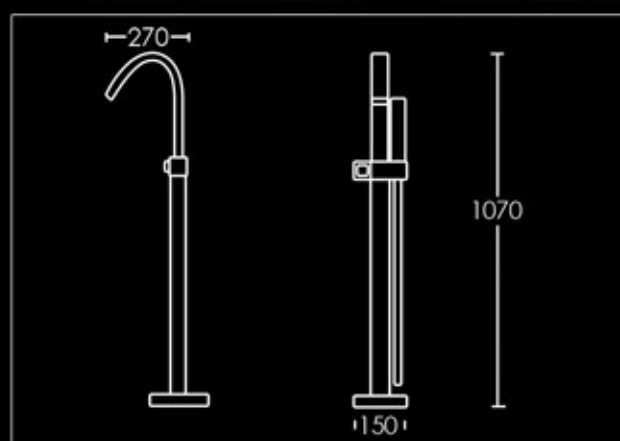
Floor Mount Bath Mixer with Slide Handshower
