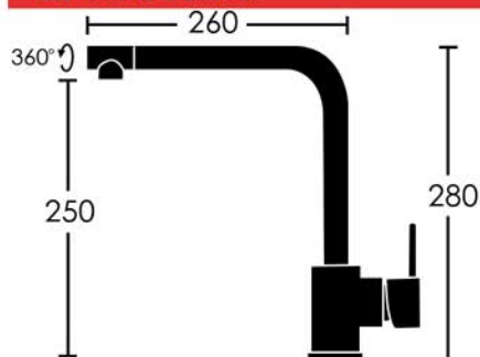
Sink Mixer
