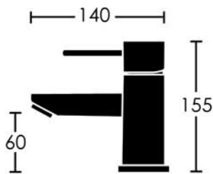
Basin Mixer
