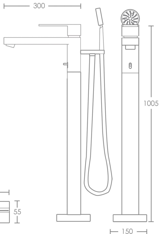
Floor Mount Bath Mixer & Handshower
