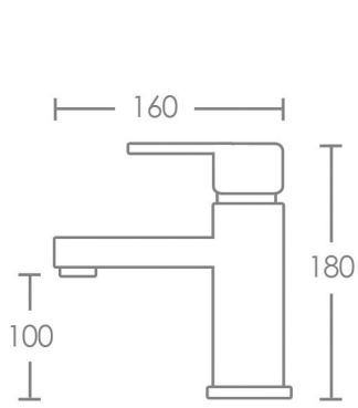
Basin Mixer
