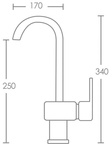
Gooseneck Sink Mixer
