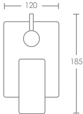
In Wall Mixer with Diverter
