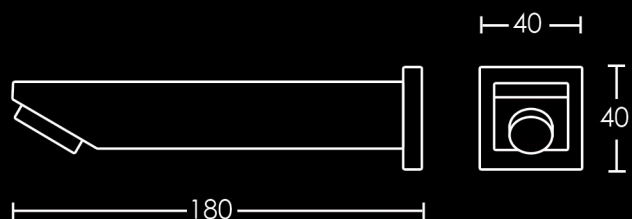
Wall Spout
