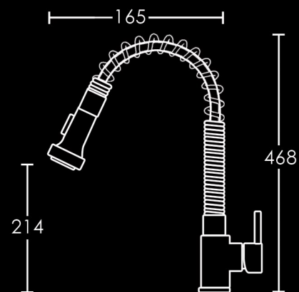
Sink Mixer
